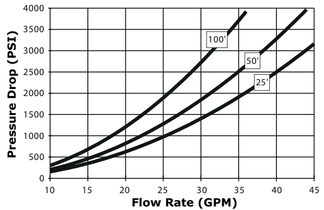
10mm Hose Pressure Drop
