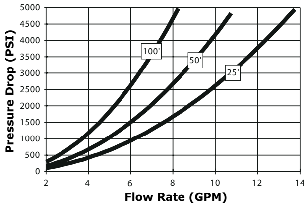
5mm Hose Pressure Drop
