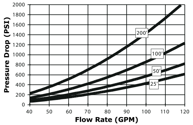
20mm Hose Pressure Drop
