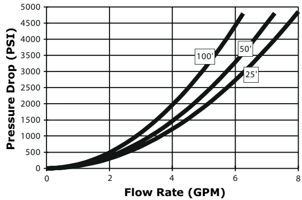
8005ST Hose Pressure Drop
