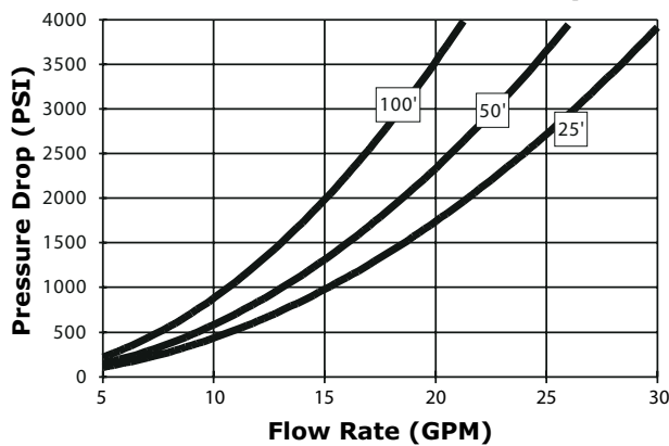
8mm Hose Pressure Drop
