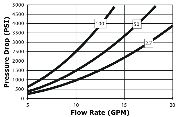
6mm Hose Pressure Drop
