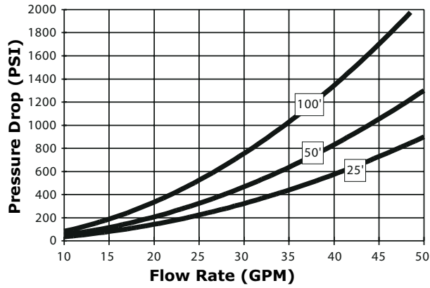
13mm Hose Pressure Drop
