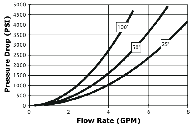
4mm Hose Pressure Drop
