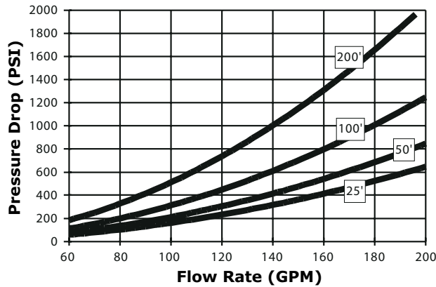
25mm Hose Pressure Drop
