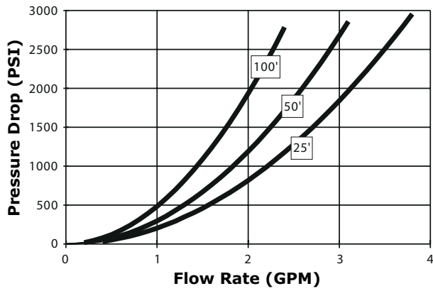
3mm Hose Pressure Drop
